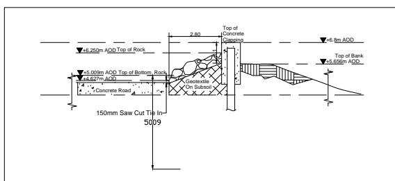
13 SECTION-13 1: 100
