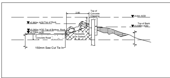
11 SECTION-11 1: 100
