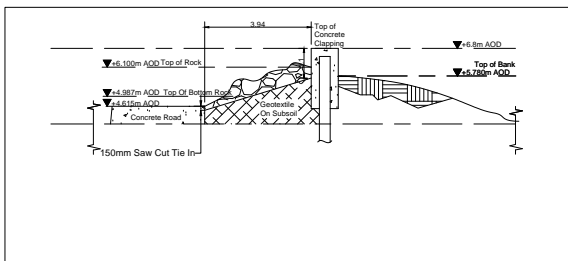
7 SECTION-7 1: 100
