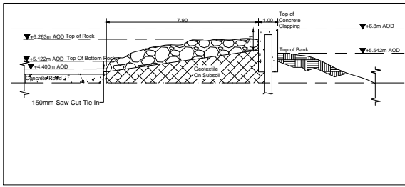
1 SECTION-1 1: 100
