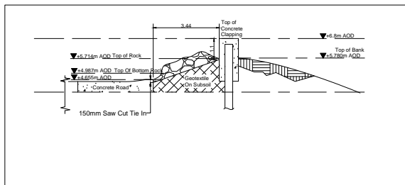
8 SECTION-8 1: 100
