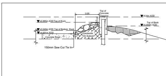
14 SECTION-14 1: 100
