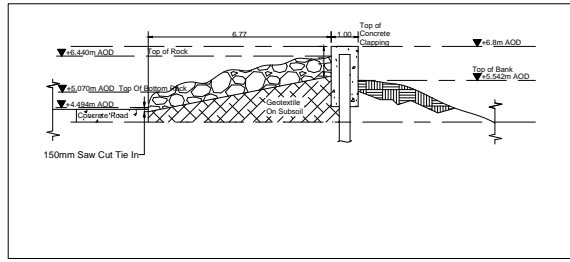
2 SECTION-2 1: 100
