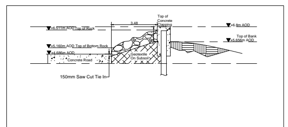
15 SECTION-15 1: 100
