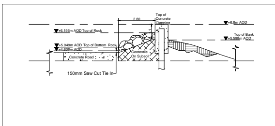
10 SECTION-10 1: 100
