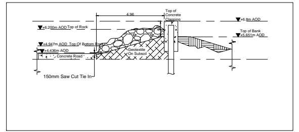
4 SECTION-3 1: 100
