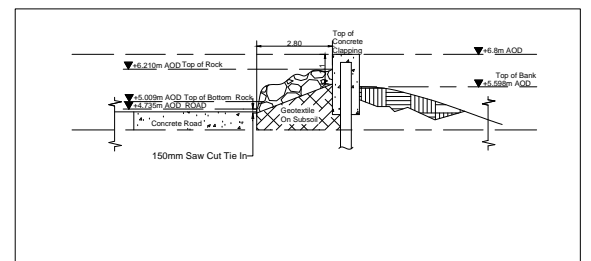
12 SECTION-12 1: 100
