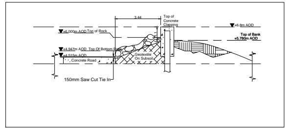
6 SECTION-6 1: 100
