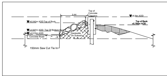
5 SECTION-5 1: 100
