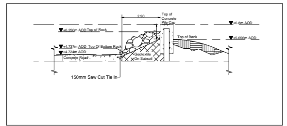
9 SECTION-9 1: 100
